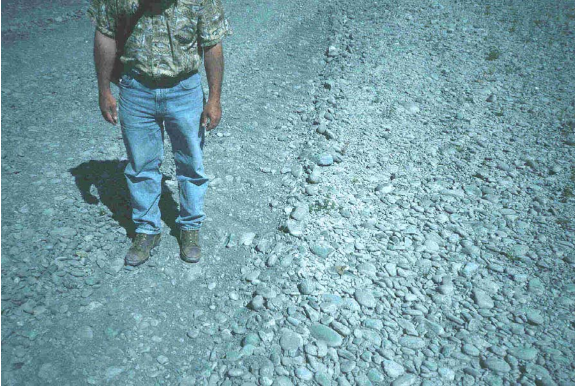
Figure 2. Photo of grain-size differences between skimmed (left) and unskimmed (right) bar surface.
