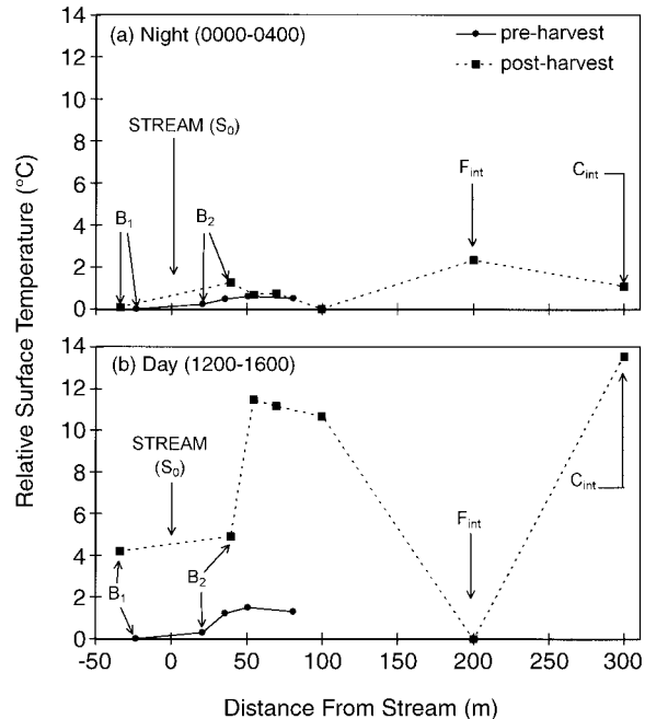
FIG. 4. Changes in average relative surface temperature [ \Delta T_{sf(i)} = T_{sf}(i) - \min[T_{sf}(1, \dots, 8)] , where T_{sf}(i) is average surface temperature at station i , and \min[T_{sf}(1, \dots, 8)] represents the minimum average surface temperature among the eight weather stations] with distance from the stream for combined pre-harvest and post-harvest sites during two time periods. Note that there are no data for the stream (distance = 0).
