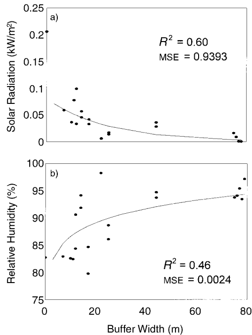
FIG. 8. Effects of buffer width on relative humidity and solar radiation at the stream. All 20 transects were used in analyses; the points grouped around 80 m represent pre-harvest data. Best-fit regression models are: R_t = \exp[-2.5186 - 0.0409 \times (\text{buffer width})] , R^2 = 0.60 ; and h = \exp[4.3671 + 0.0412 \times \ln(\text{buffer width})] , R^2 = 0.46 .
