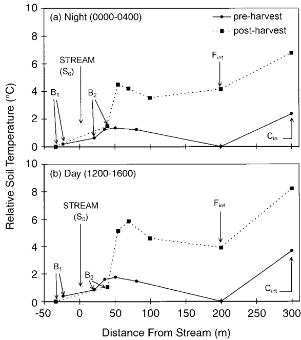
FIG. 3. Changes in average relative soil temperature [ \Delta T_{s(i)} = T_s(i) - \min[T_s(1, \dots, 8)] , where T_s(i) is average soil temperature at station i , and \min[T_s(1, \dots, 8)] represents the minimum average soil temperature among the eight weather stations] with distance from the stream for combined pre-harvest and post-harvest sites during two time periods. Note that there are no data for the stream (distance = 0).
